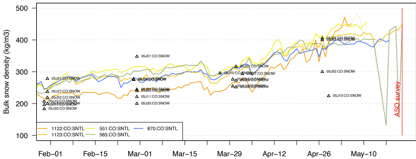
Figure 4. Daily snow density timeseries at automated sensor locations in the Poudre Basin and neighboring basins. (Data source: NRCS)
