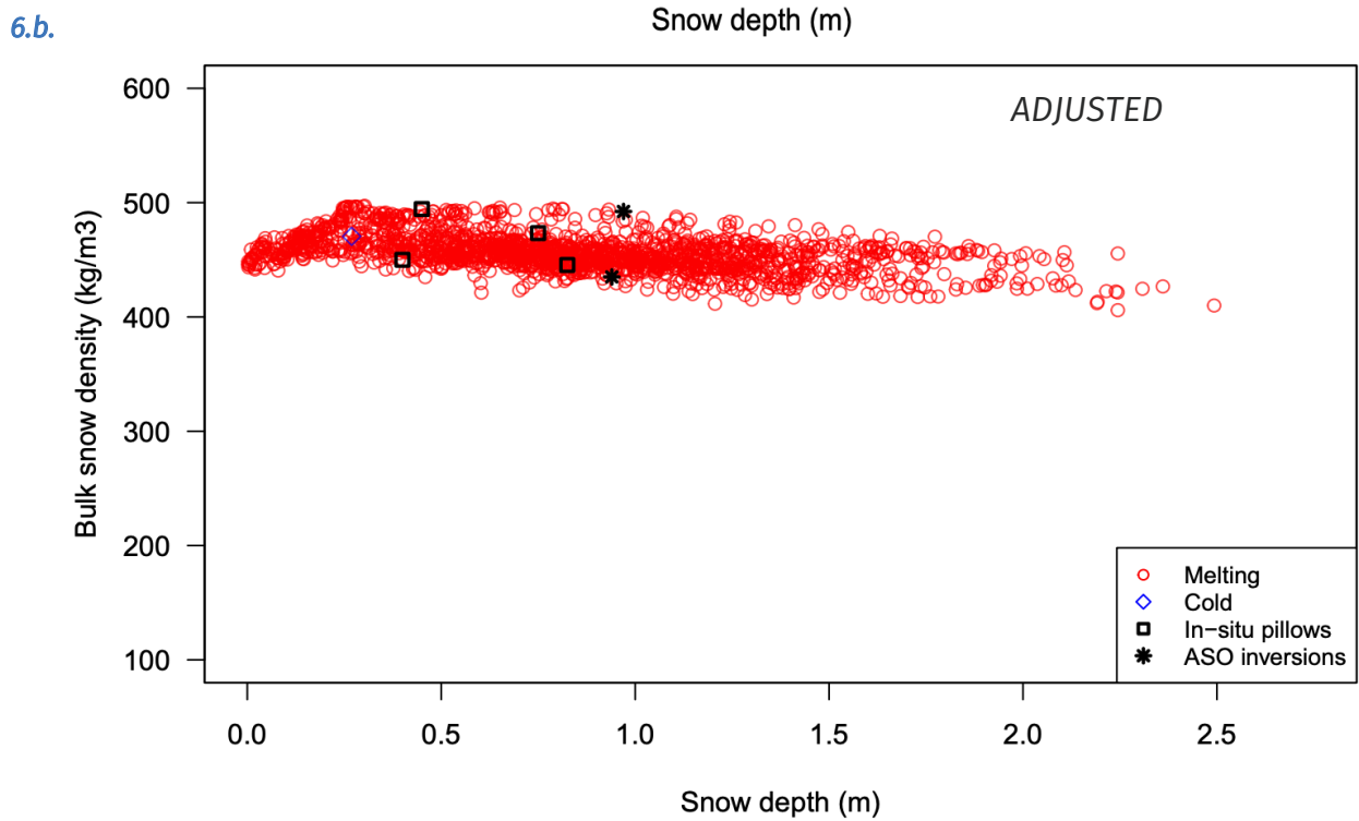
Figure 6. Observed and modeled bulk snow density (kg/m 3 ) by snow depth (m) for a. open-loop and b. adjusted densities. Red circles represent modeled densities of melting snow (cold content = 0), blue diamonds represent modeled densities of cold snow (cold content < 0).
