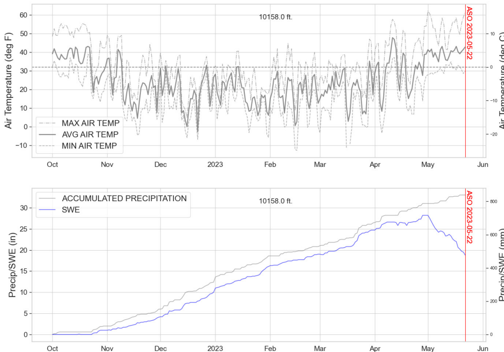
Figure 3. Daily meteorological conditions at Joe Wright SNOTEL (551) (elevation 10158 ft). Note: the raw daily data shown has been downloaded directly from NRCS and has not been quality checked. There may be noise or incorrect data present. Precipitation data will only be shown if the featured station records it, and the air temperature plot shows daily max, mean, and min values. ASO surveys are marked with red vertical lines.
