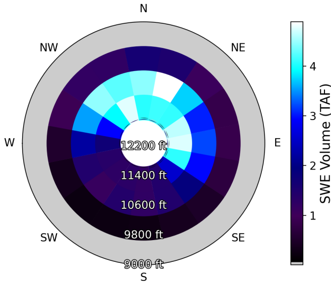
Figure 7.a. & 7.b. SWE volume (TAF) and depth (m) by aspect and elevation for May 22 survey.
