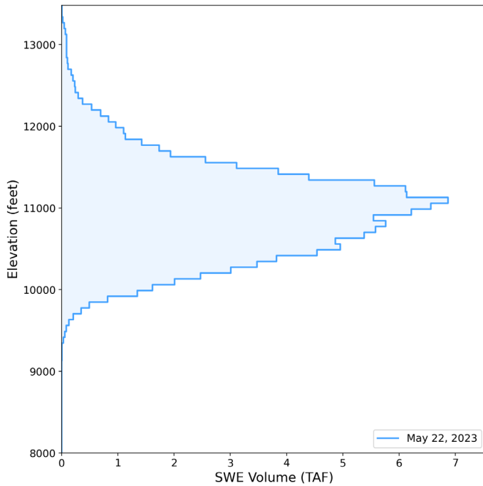
Figure 8.a. Distribution of SWE volume (TAF) across elevations for the May 22 survey. 8.b. Distribution of SWE depth (in) across elevations; solid line represents median SWE depth (in), lighter color bands represent the 25th to 75th percentile.
