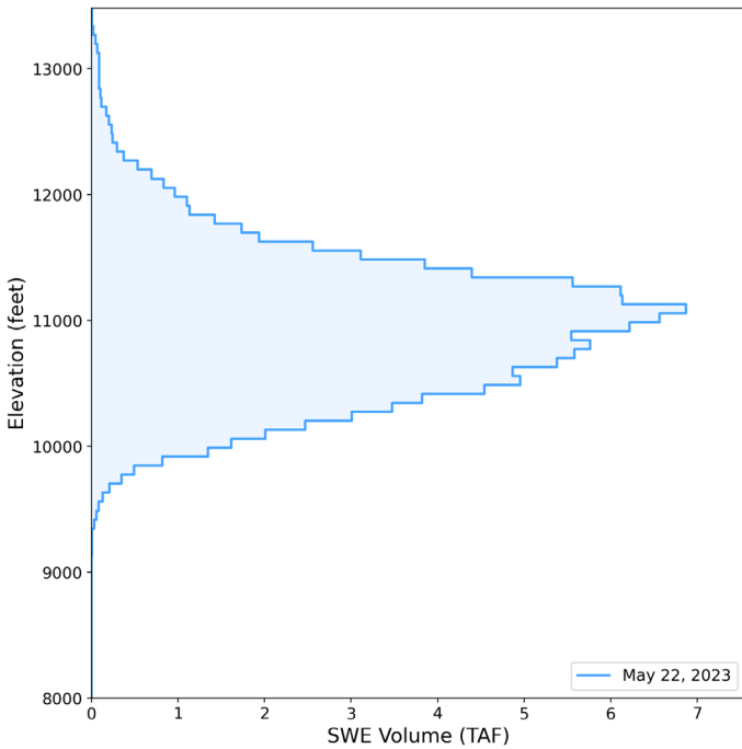
Figure 2.a. Distribution of SWE volume (TAF) across elevations. Figure 2.b. Distribution of SWE volume (TAF) by aspect and elevation for the May 22 survey. See Figure 7 and Figure 8 for more descriptive plots.
