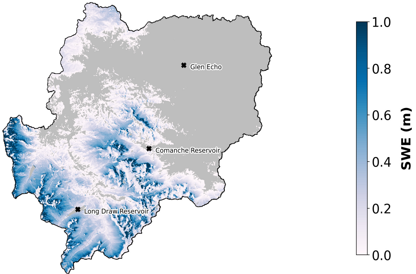
Figure 1. Spatial distribution of SWE depth (m).
