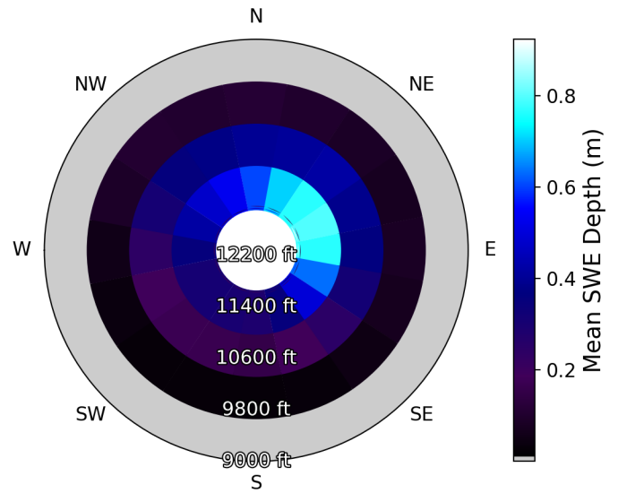
Figure 7.a. & 7.b. SWE volume (TAF) and depth (m) by aspect and elevation for May 22 survey.
