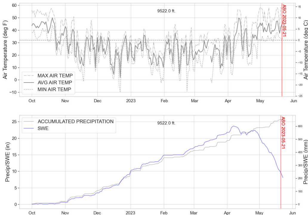
Figure 3. Daily meteorological conditions at Bear Lake (322) (elevation 9522 ft). Note: the raw daily data shown has been downloaded directly from NRCS and has not been quality checked. There may be noise or incorrect data present. Precipitation data will only be shown if the featured station records it, and the air temperature plot shows daily max, mean, and min values. ASO surveys are marked with red vertical lines.
