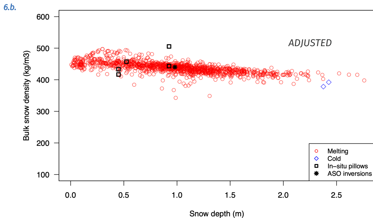
Figure 6. Observed and modeled bulk snow density ( \text{kg/m}^3 ) by snow depth (m) for a. open-loop and b. adjusted densities. The black stars represent the density inversions described in Sensor Measurements . Red circles represent modeled densities of melting snow (cold content = 0), blue diamonds represent modeled densities of cold snow (cold content < 0).
