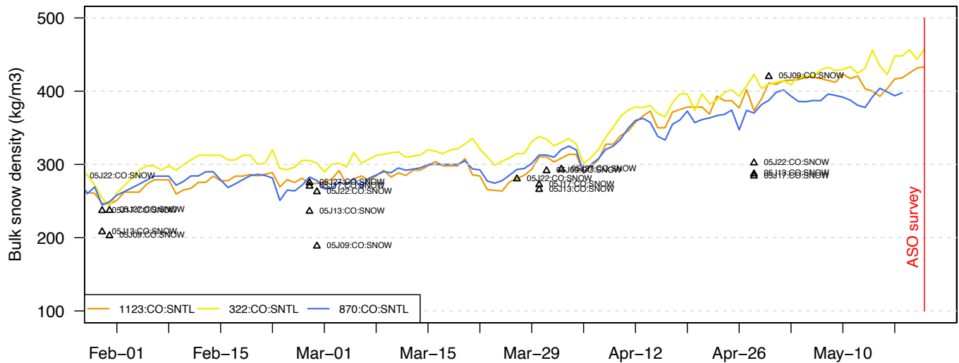
Figure 4. Daily snow density timeseries at automated sensor locations in the Big & Little Thompson River Basins and neighboring basins. (Data source: NRCS)
